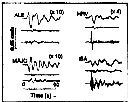
Fig. 4. Broad-band velocity records from four stations (ALE: epicentral distance \Delta = 5185 km, azimuth = 9^\circ ; HRV: \Delta = 4366 km, azimuth = 68^\circ ; MAJO: \Delta = 8029 km, azimuth = 305^\circ ; ISA: \Delta = 745 km, azimuth = 132^\circ ) for the main shock (top trace) and the first (middle) and second (lower) aftershocks. The amplitudes of the seismograms at ALE, HRV, and MAJO are increased relative to ISA for display. The large amplitudes of the second aftershock relative to the other two events in the along-strike azimuth (ISA) is attributable to rupture directivity.
